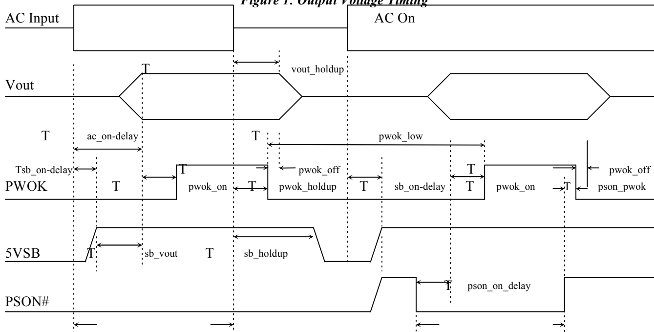
Figure 1: Output Voltage Timing
